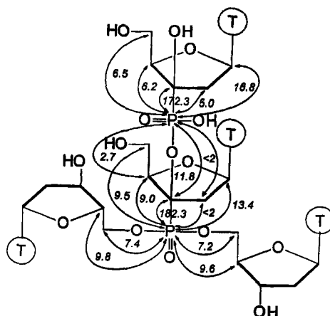
FIGURE 1 Phosphorus-carbon coupling constants in compound 14
